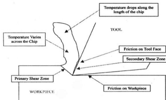
Fig.1 Heat generated during turning CHIP MORPHOLOGY
