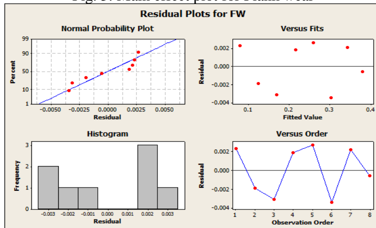
Fig. 6: Residual plot for Flank wear
